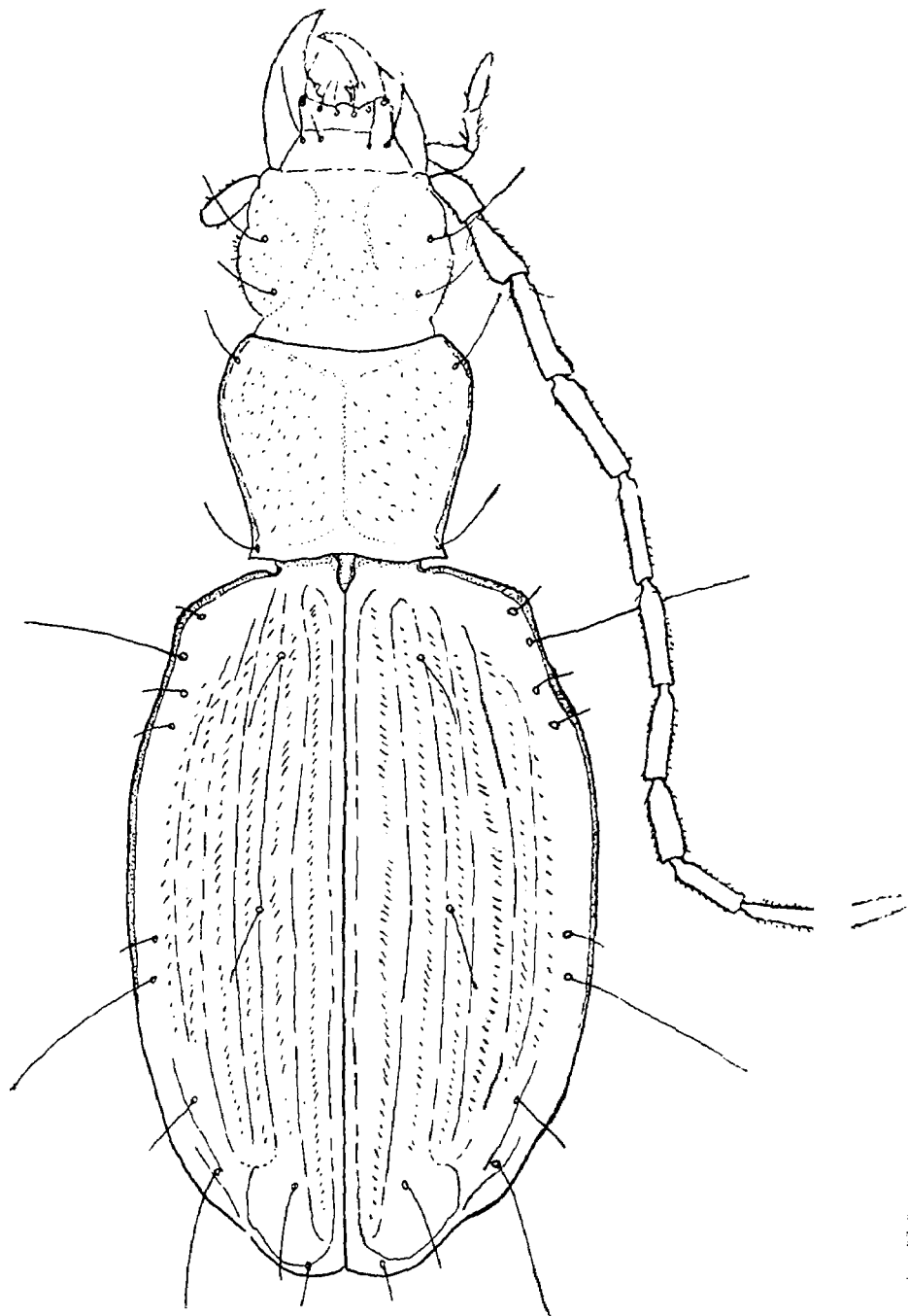
FIGURE 1. Pseudanophthalmus orlindae n. sp. Holotype male, X23.
